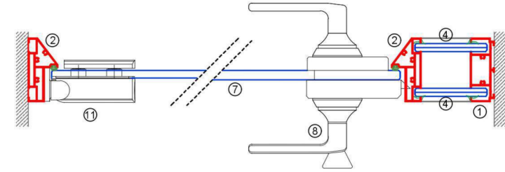
ALTERNATIVE DOOR WITH HYDRAULIC HINGES
