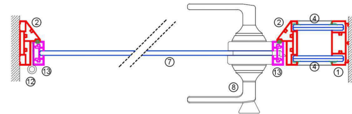
ALTERNATIVE DOOR WITH FRAMED GLASS WINGS
